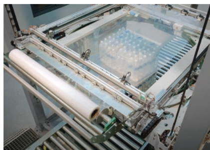
○ Top Cover: Dustproof and Rainproof
